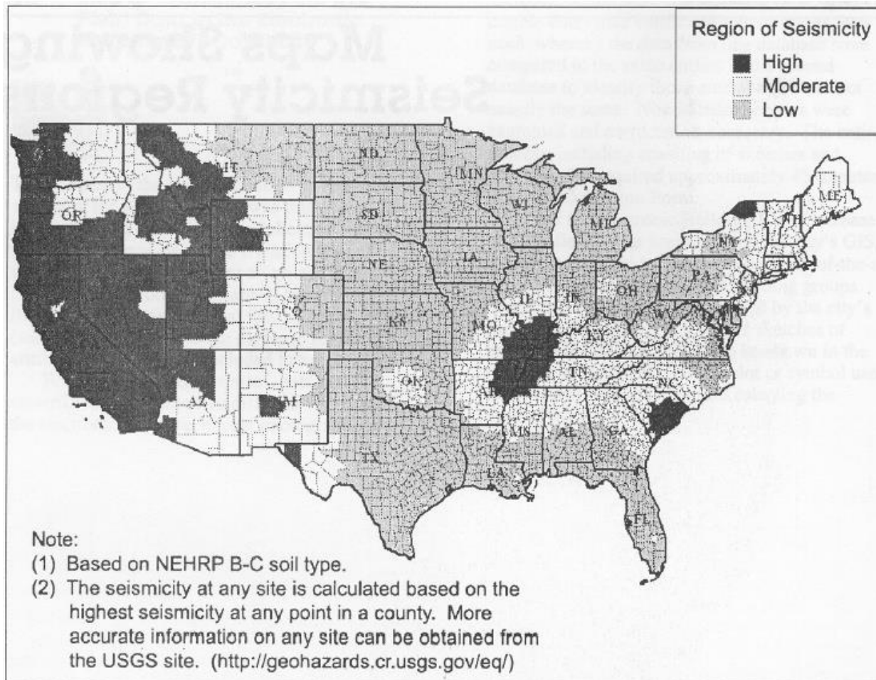
Figure 3-1. Seismic Hazard Map (FEMA, 2002b; ATC, 2002)
