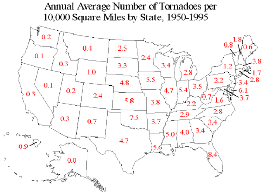
Figure 3-4. Annual Number of Tornadoes per 10,000 Square Miles, by State (NOAA, 1999)
